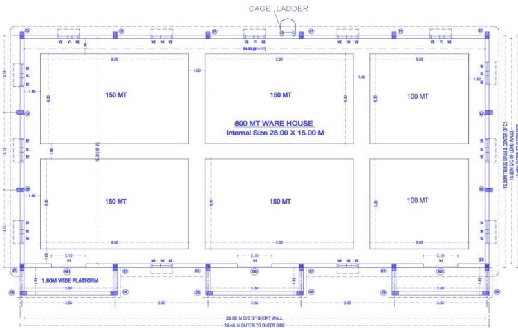
800 MT WARE HOUSE UNIT PLAN
